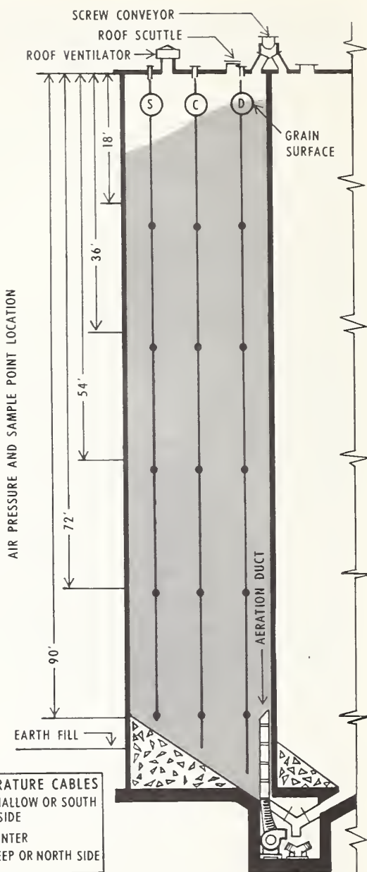
FIGURE 4.—Grain aeration system layout for test of experimental vertical aeration duct. Section of concrete storage annex with round tanks of 20-foot diameter and 100-foot maximum depth.
